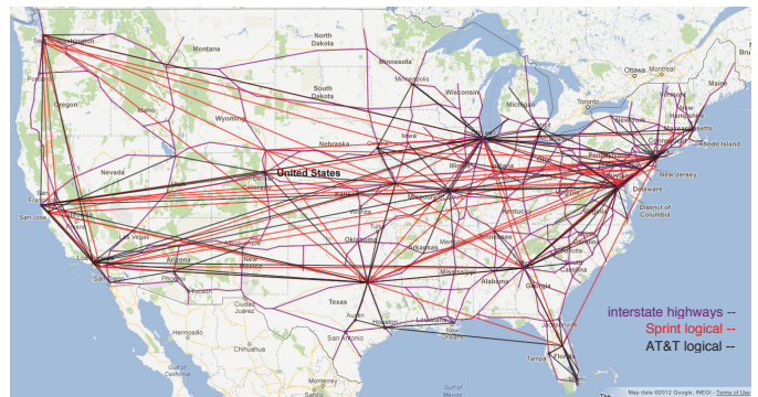
Fig. 2. Logical topologies overlaid on highways
