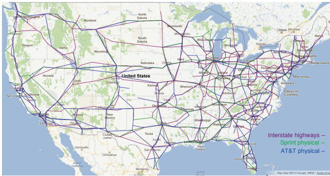
Fig. 3. Physical topologies overlaid on highways
